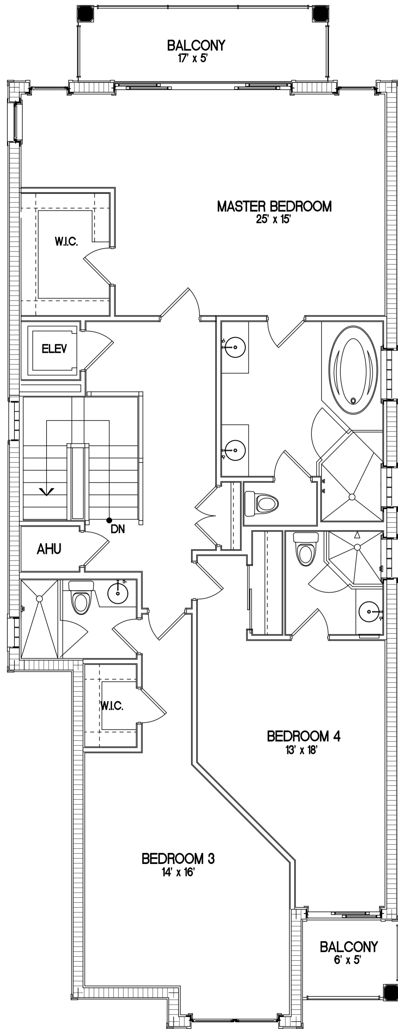
SECOND FLOOR
