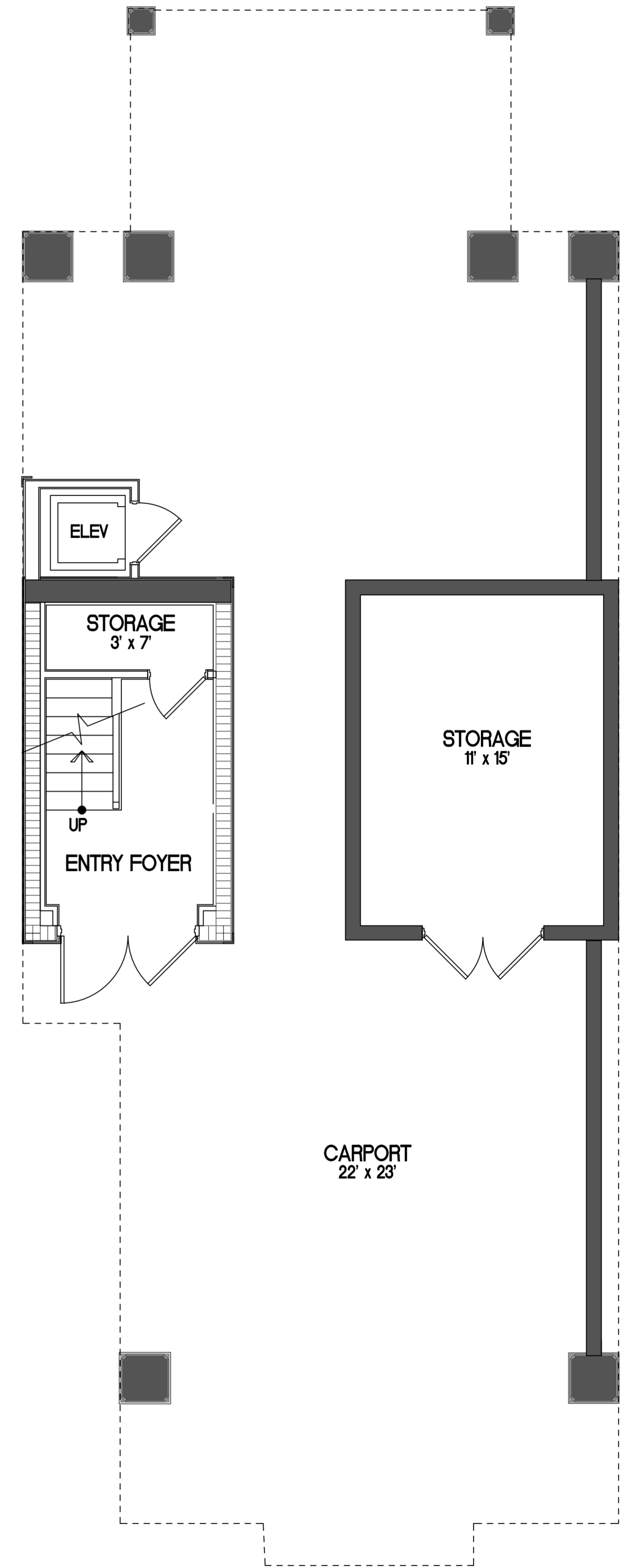
GROUND FLOOR
